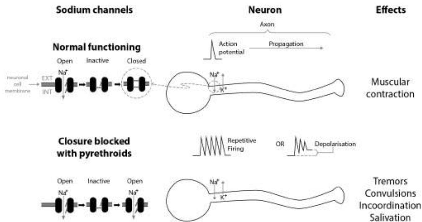
Figure 3: Pyrethroids' mode of action on neurons.
