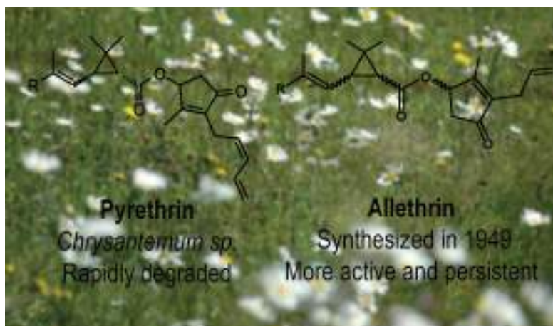
Figure 1: Comparison of pyrethrin, extracted from chrysanthemum flowers, and allethrin, the first synthesized pyrethroid.
